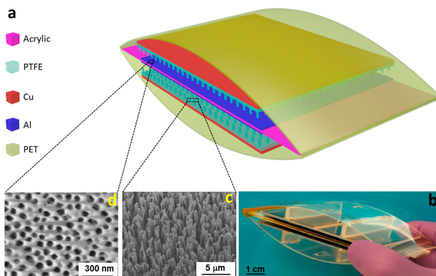
Figure 1. Single unit in a TENG. (a) Schematic illustration and (b) photograph of an as-fabricated minimum functional unit. (c) SEM image of PTFE nanowires. (d) SEM image of nanopores on aluminum electrode.
